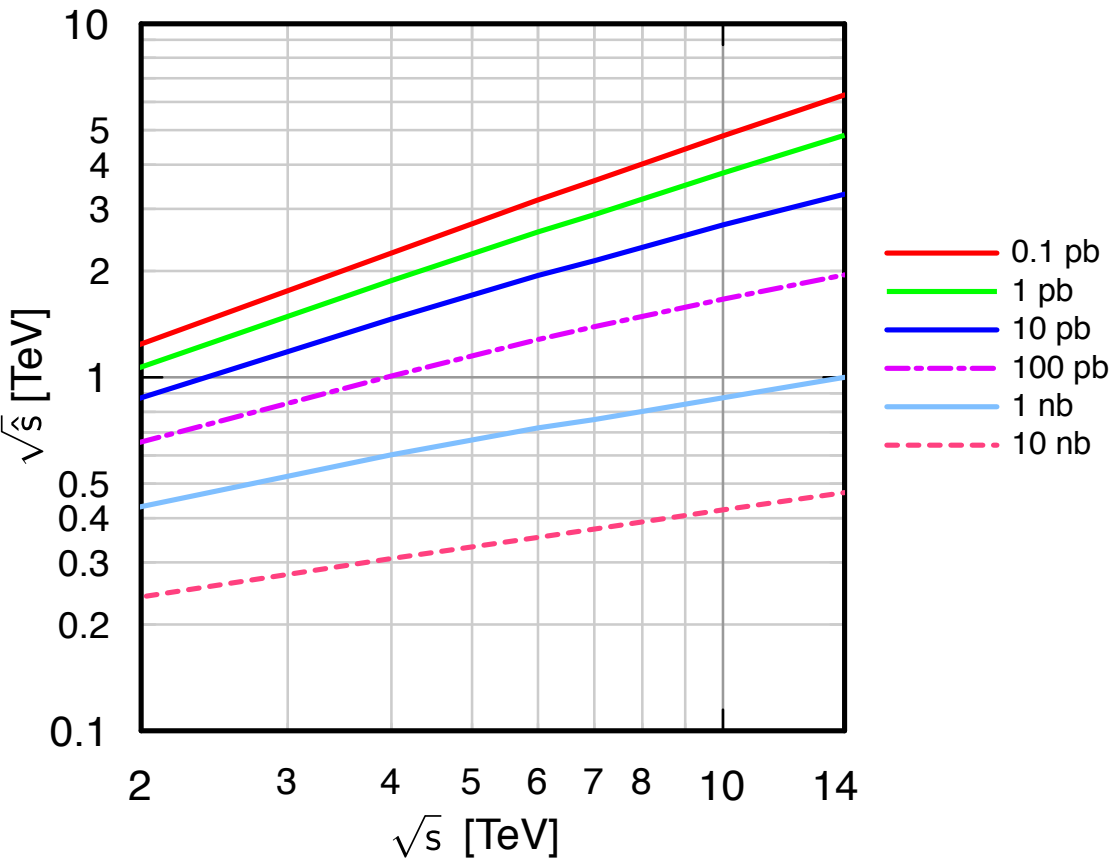
CTEQ6L1: qq
